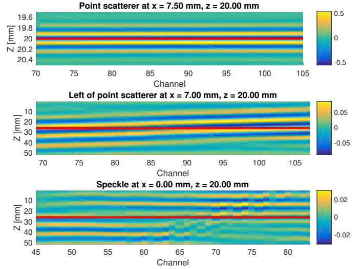
Fig. 5: The delayed wavefield for three different pixels in Fig. 1. The top is from the point scatterer at x = 7.5 mm and z = 20 mm, the middle to the left of the point scatterer at x = 7 mm and z = 20 and the bottom from the speckle pattern at x = 0.0 mm and z = 20 mm. The red line in the plot indicates the signals contributing in the sum of "delay-and-sum" beamforming when estimating the amplitude in the pixel.
