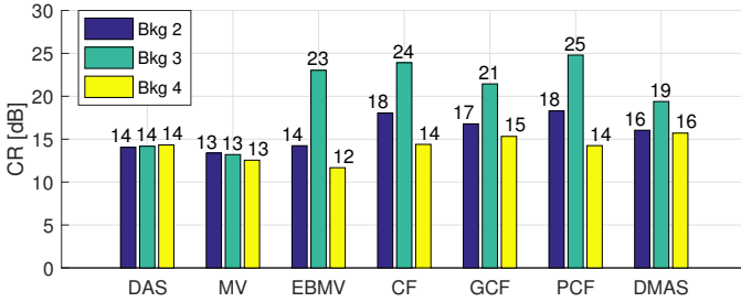
Fig. 4: Measured contrast ratio difference for the experimental dataset shown in Fig. 3. The CR was measured between the cyst, region 1 in Fig. 3a, and background region 2, 3 and 4.
