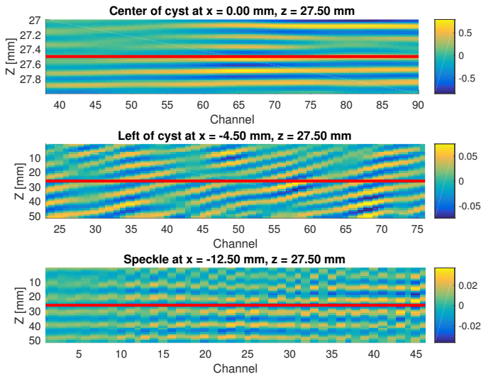
Fig. 6: The delayed wavefield for three different pixels in Fig. 3. The top is for the pixel at x = 0.0 mm and z = 27.5 mm inside the hyperechoic cyst, the middle is for the pixel at x = -4.5 mm and z = 27.5 mm to the left of the hyperechoic cyst, and the lower plot is for the pixel in speckle at x = -12.5 mm and z = 27.5 mm. The red line in the plot indicates the signals contributing in the sum of "delay-and-sum" beamforming when estimating the amplitude in the pixel.
