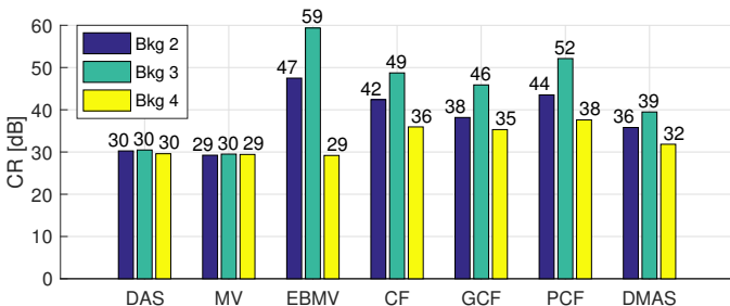
Fig. 2: Measured contrast ratio difference for the simulated dataset shown in Fig. 1. The CR was measured between the cyst, region 1 in Fig. 1a, and background region 2, 3 and 4.
